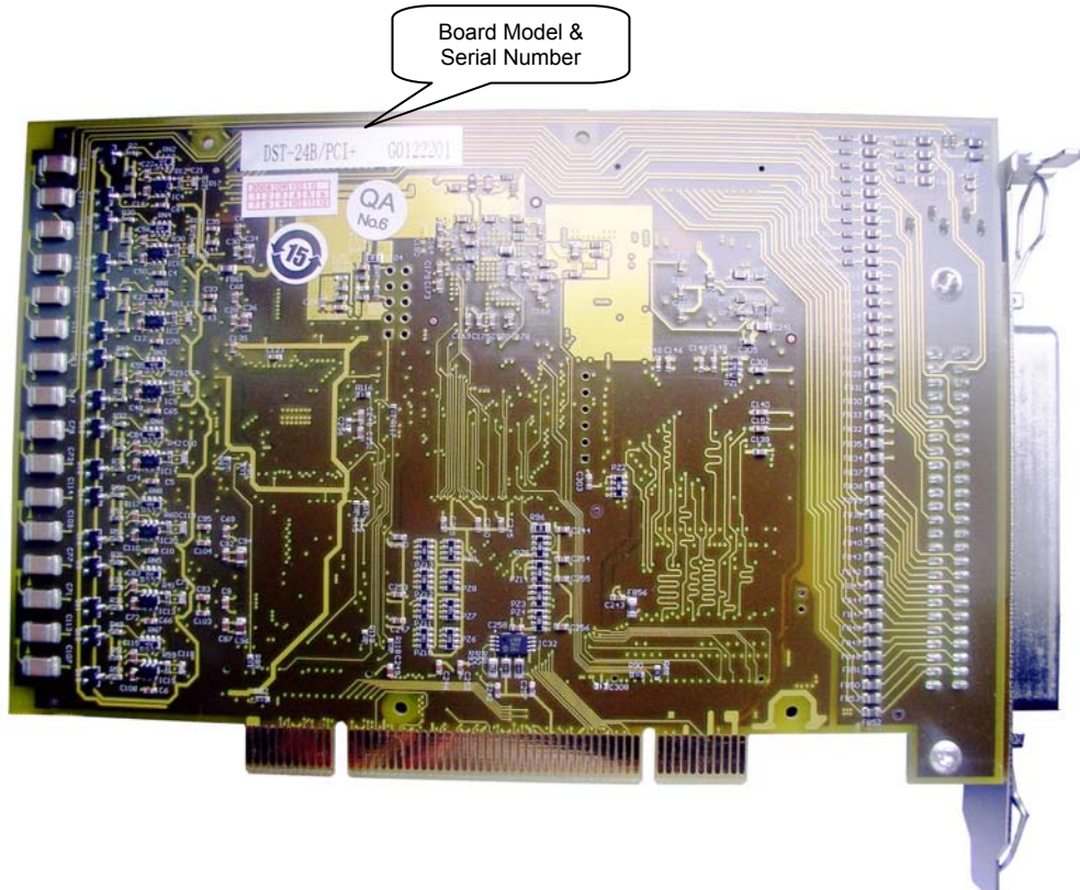
Figure 2-6 DST-24B/PCI(2.0), DST-24B/PCI+(2.0) (Rear View)
