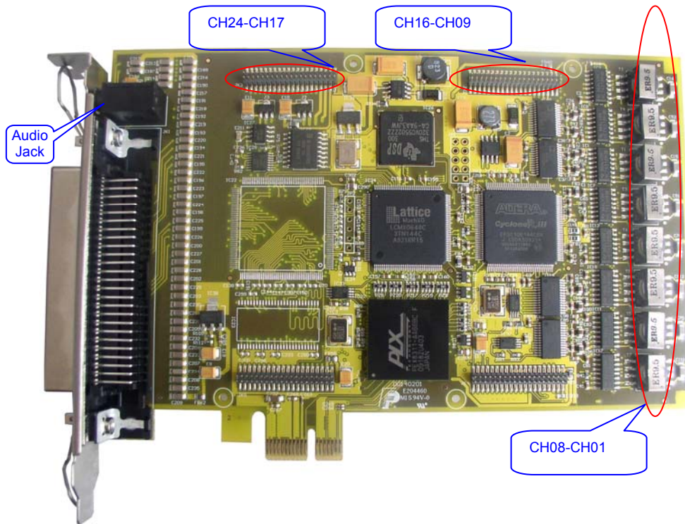
Figure 2-7 DST-24B/PCle(2.0)(Front View)
