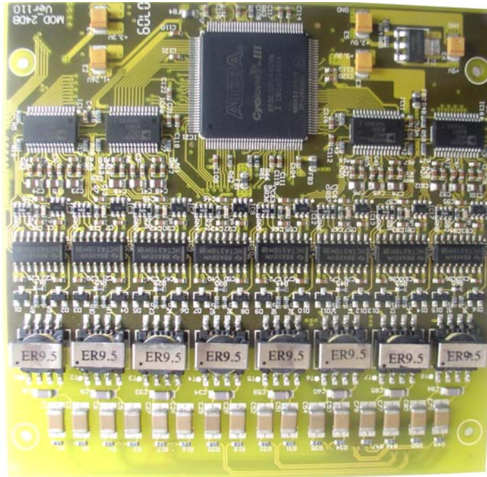
Figure 2-10 MOD-24DB (Version 1.10)
